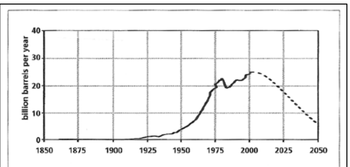
FIGURE 3-12 Scenario for Global Oil Production
