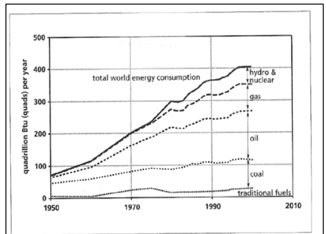
FIGURE 3-10 World Energy Use
