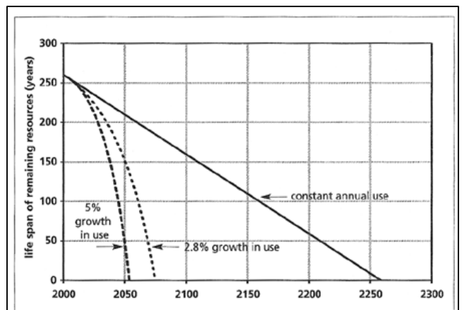
FIGURE 3-13 Some Possible Paths of World Gas Depletion
